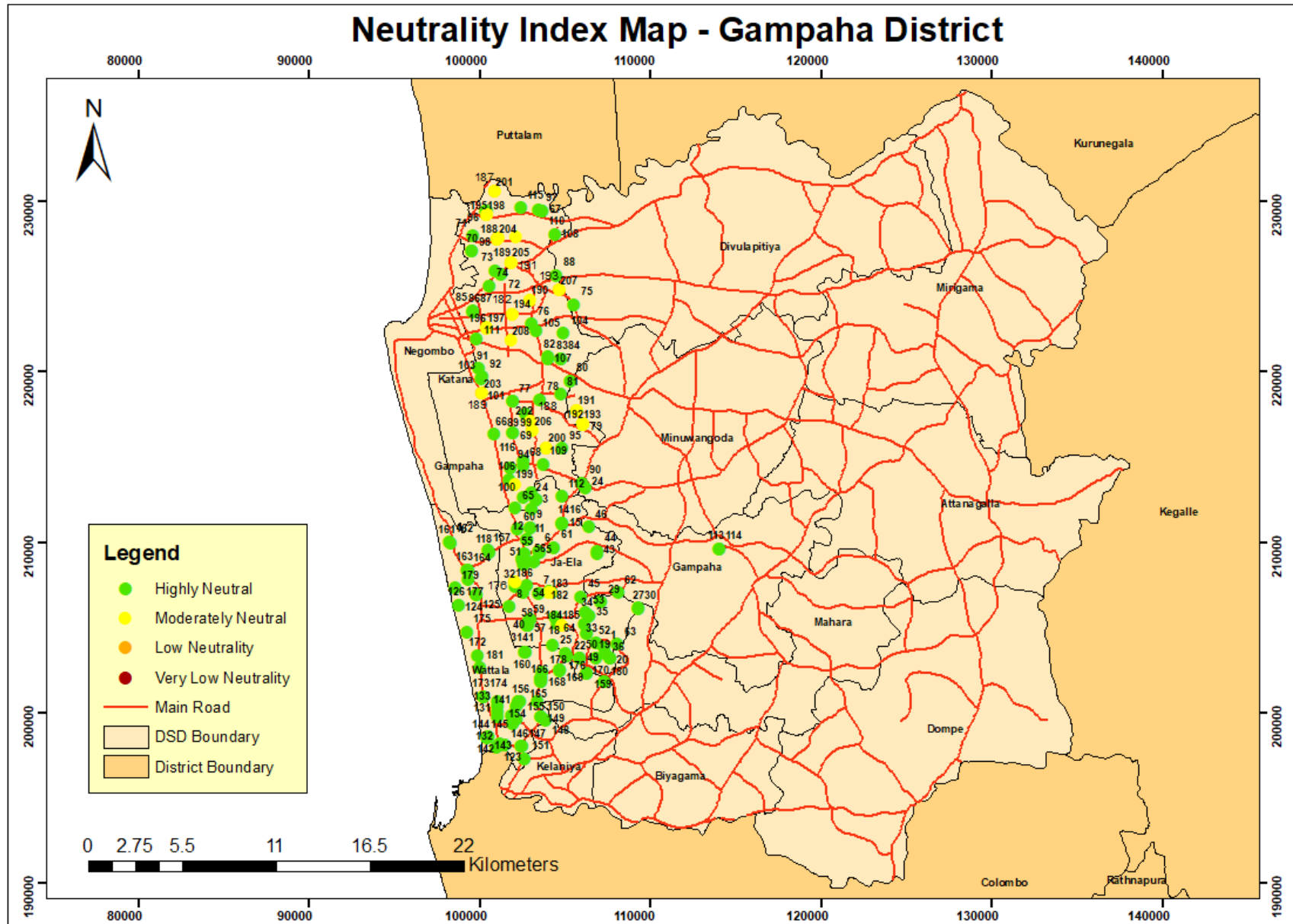
Figure 3.2: Neutrality Index Map
